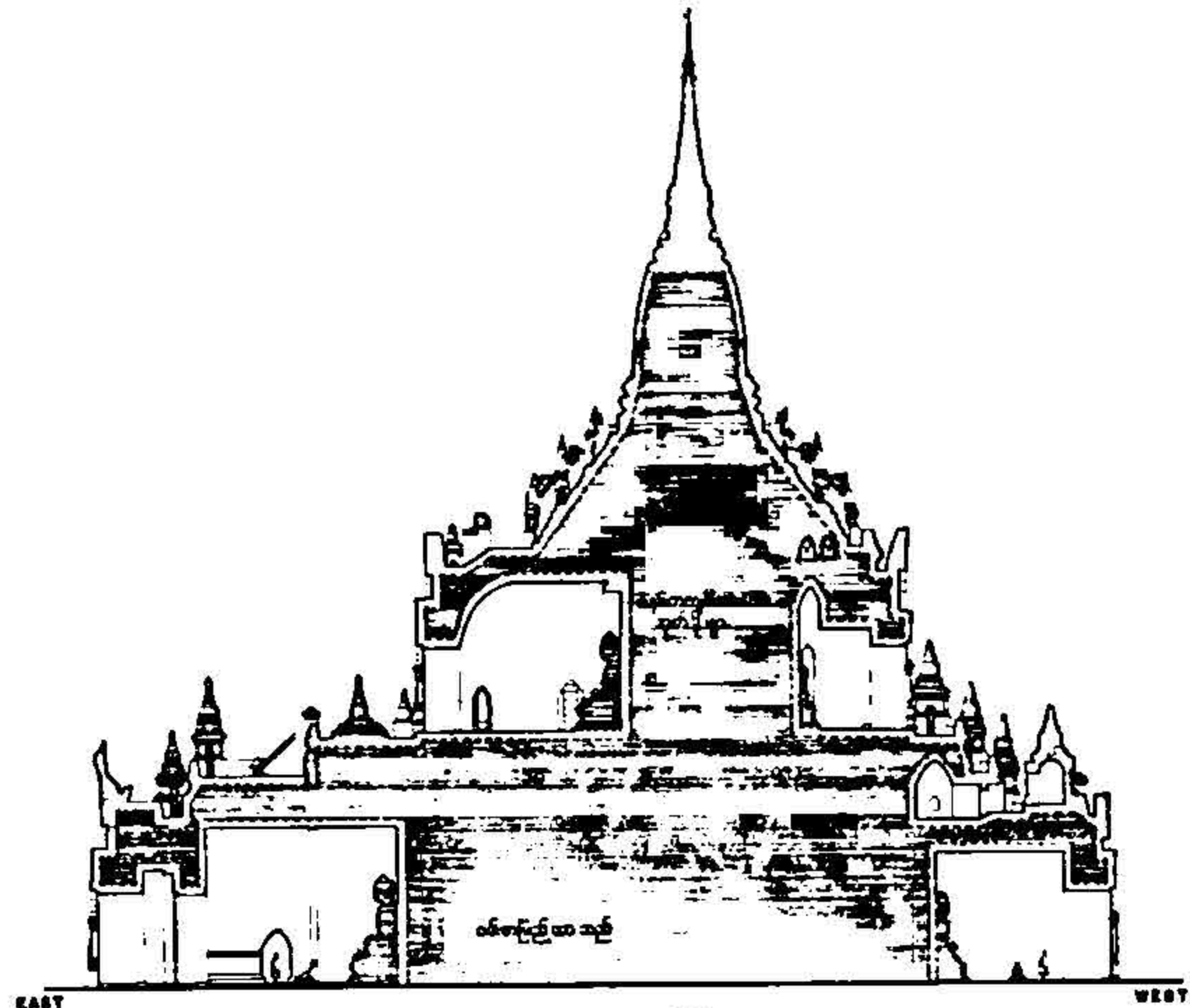
GAWDAWPALIN. BUILT BY NARAPATISITHU 1175 - 1210 A.D. SECTION THROUGH EAST WEST. DEPARTMENT OF ARCHITECTURE RANGOON INSTITUTE OF TECHNOLOGY
