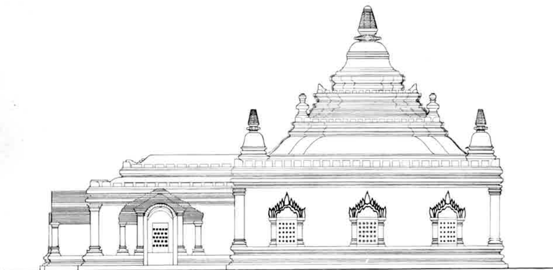
ABEYADANA TEMPLE west elevation
